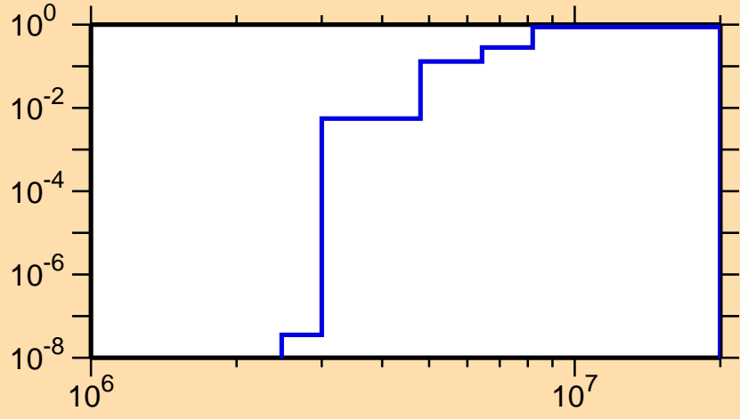
\sigma vs. E for ^{183}\text{Tl}(n,np)
