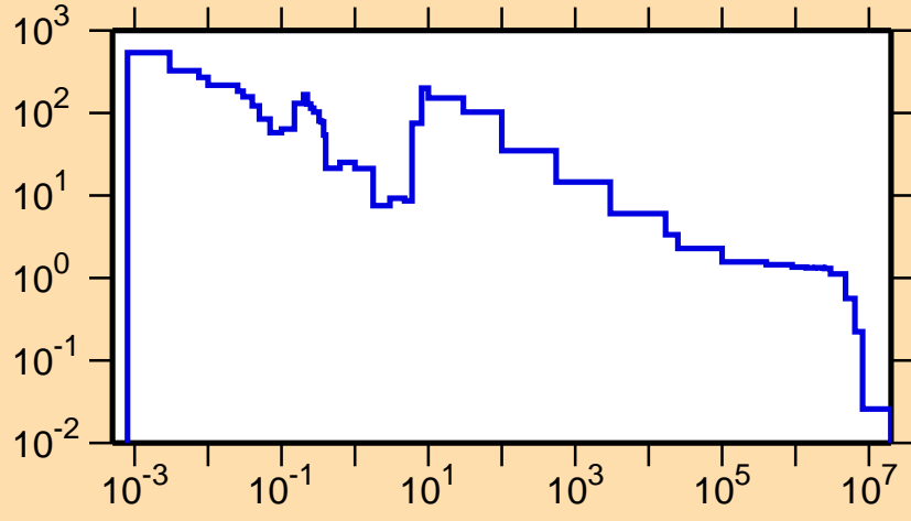
\sigma vs. E for ^{183}\text{Tl}(n,\gamma)
