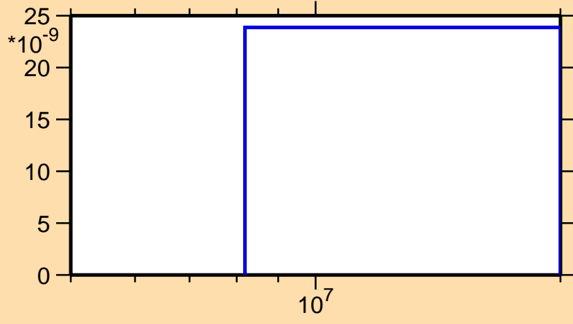
\sigma vs. E for ^{183}\text{Tl}(n,nd)
