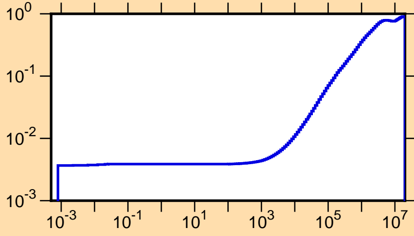
\mu vs. E for ^{184}\text{Tl}(\text{mt251})
