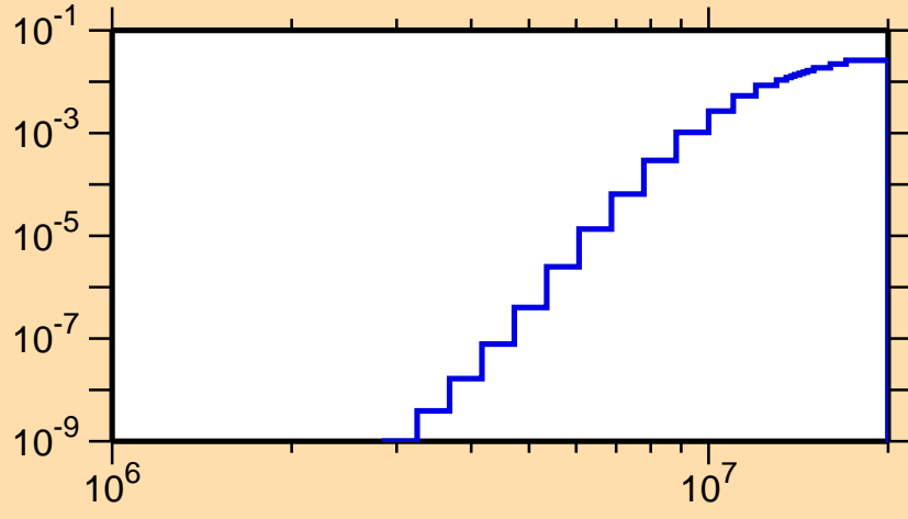
\sigma vs. E for ^{184}\text{Tl}(n,d)
