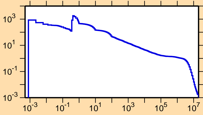
\sigma vs. E for ^{184}\text{Tl}(n,\gamma)
