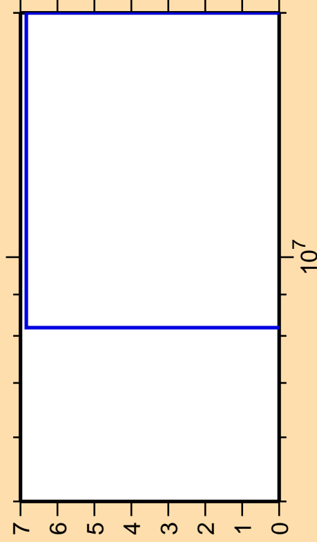
\Delta\sigma/\sigma vs. E for ^{184}\text{Tl}(n,3n)
