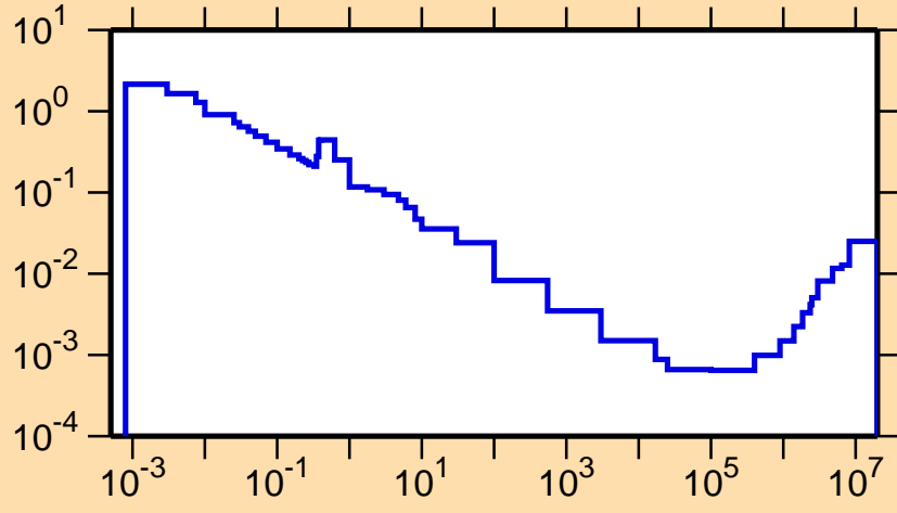
\sigma vs. E for ^{184}\text{Tl}(n,p\alpha)
