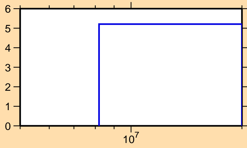
\Delta\sigma/\sigma vs. E for ^{184}\text{Tl}(n,\text{el.})
