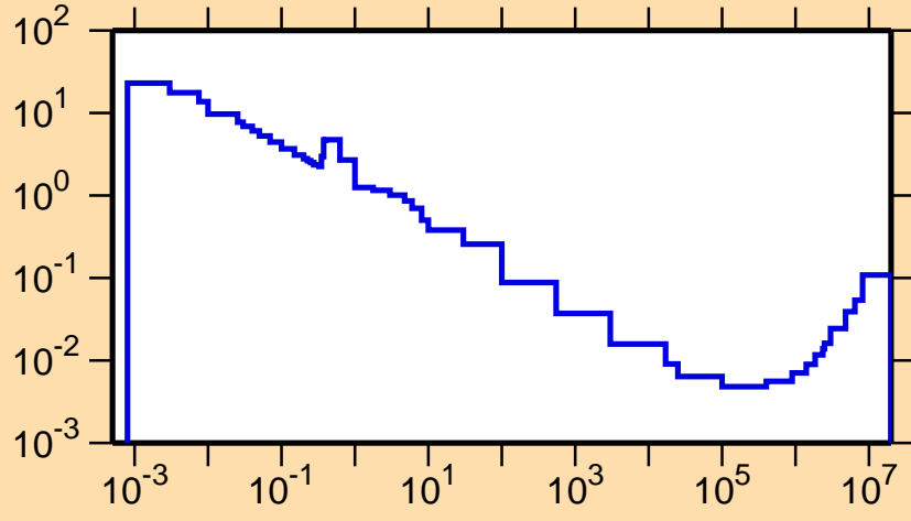
\sigma vs. E for ^{184}\text{Tl}(n,\alpha)
