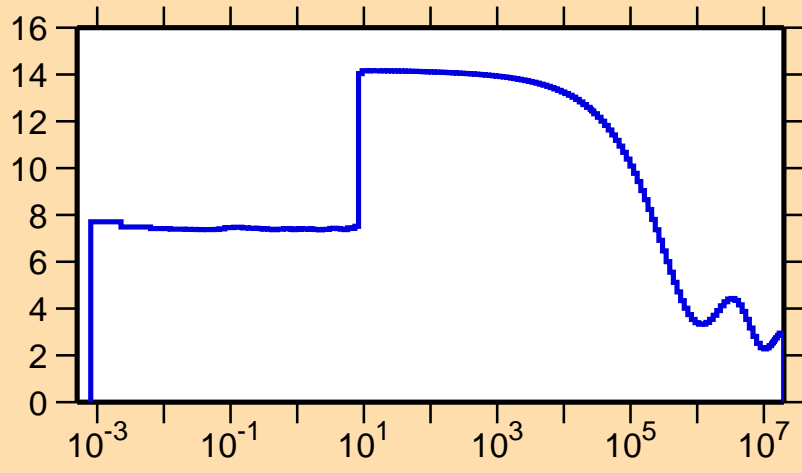
\sigma vs. E for ^{185}\text{Tl}(n,\text{el.})
