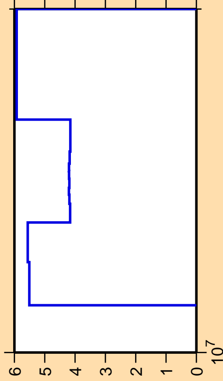
\Delta\sigma/\sigma vs. E for ^{185}\text{Tl}(n,n_1)
