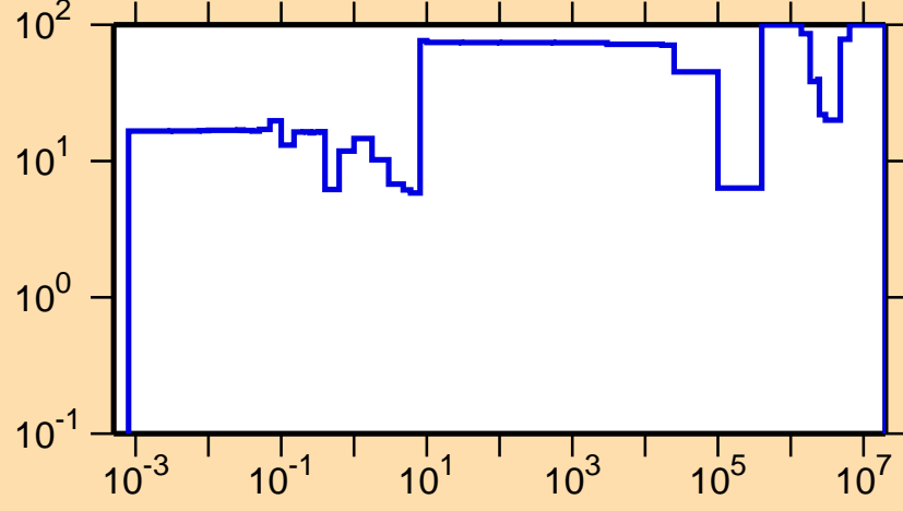
\Delta\sigma/\sigma vs. E for ^{185}\text{Tl}(n,el.)
