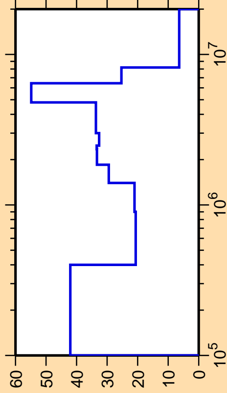
\Delta\sigma/\sigma vs. E for ^{185}\text{Tl}(n,n_2)
