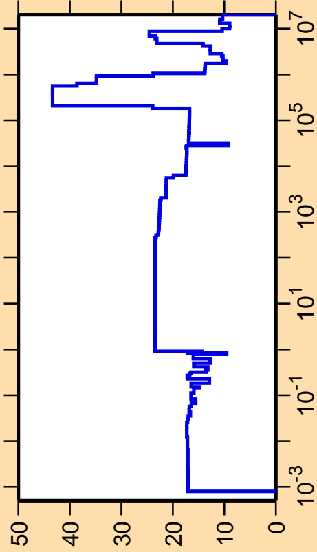
\Delta\sigma/\sigma vs. E for ^{186}\text{Tl}(n,\text{el.})
