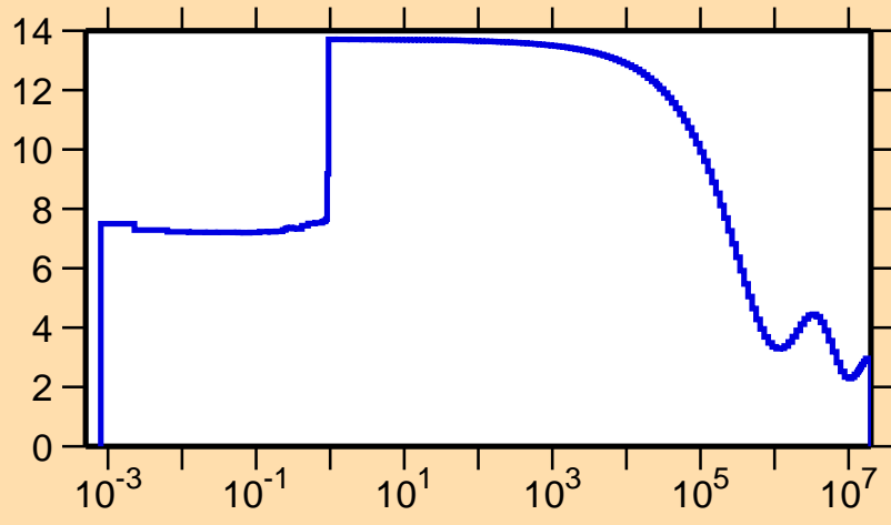
\sigma vs. E for ^{186}\text{Tl}(n,\text{el.})
