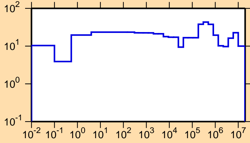
\Delta\sigma/\sigma vs. E for ^{186}\text{Tl}(n,el.)
