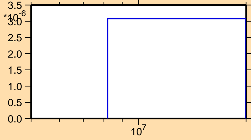
\sigma vs. E for ^{186}\text{Tl}(n,nd)
