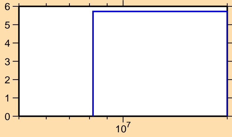
\Delta\sigma/\sigma vs. E for ^{186}\text{Tl}(n,\text{nonel.})
