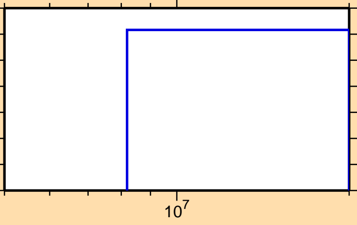
\sigma vs. E for ^{186}\text{Tl}(n,nd)
