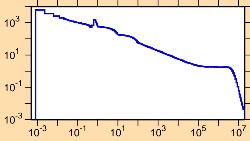
\sigma vs. E for ^{186}\text{Tl}(n,\gamma)
