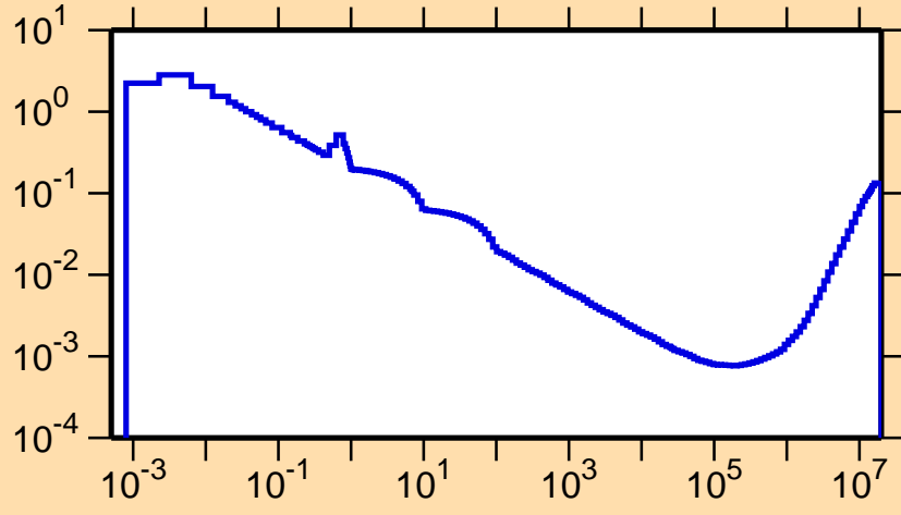
\sigma vs. E for ^{186}\text{Tl}(n,\alpha)
