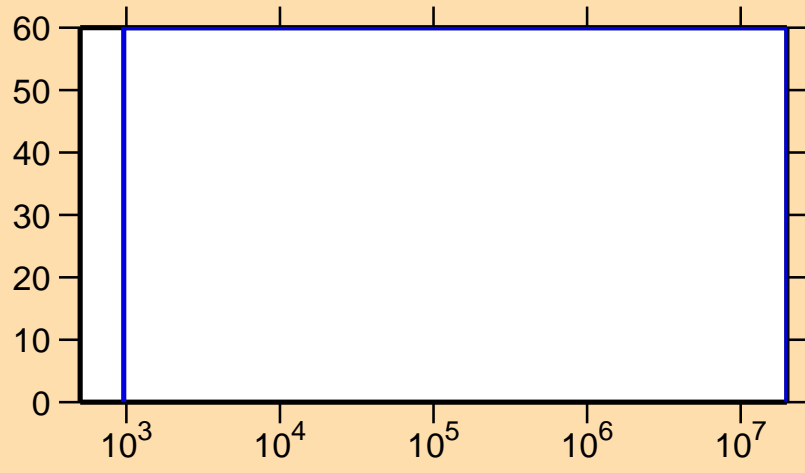
\Delta\sigma/\sigma vs. E for ^{186}\text{Tl}(n,n\text{cont.})
