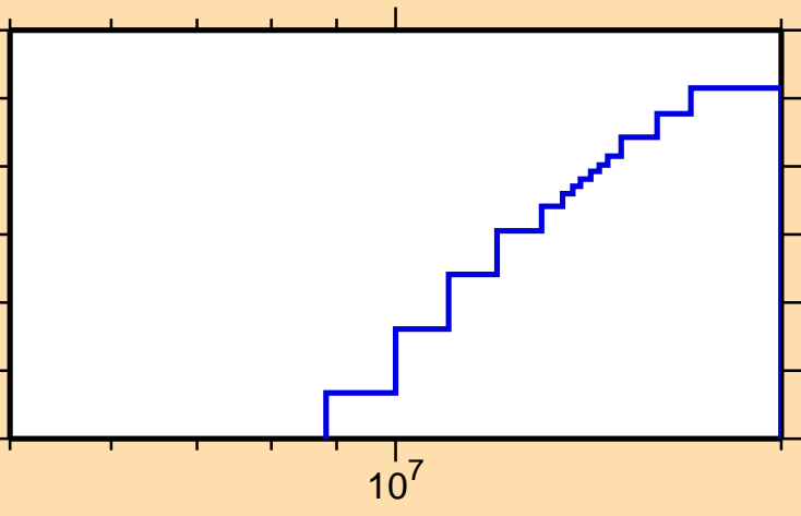
\sigma vs. E for ^{187}\text{Tl}(\text{mt117})
