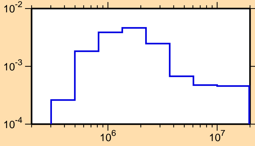
\sigma vs. E for ^{187}\text{Tl}(n,n_2)
