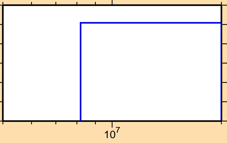
\sigma vs. E for ^{187}\text{Tl}(n,2np)
