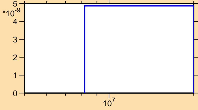
\sigma vs. E for ^{187}\text{Tl}(n,3n\alpha)
