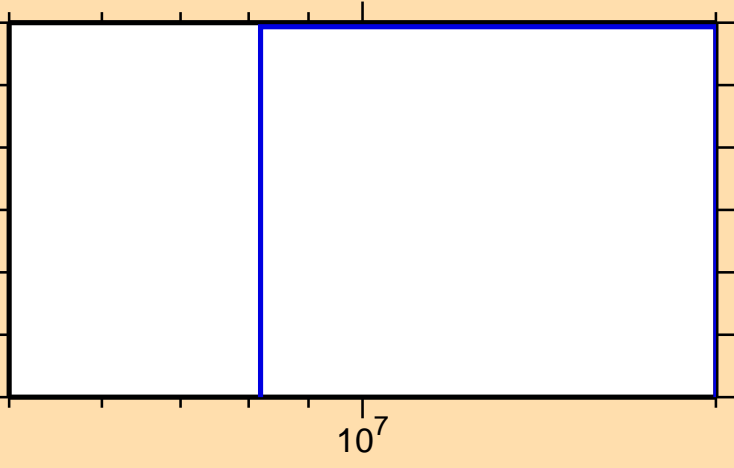
\sigma vs. E for ^{187}\text{Tl}(n,\text{pd})
