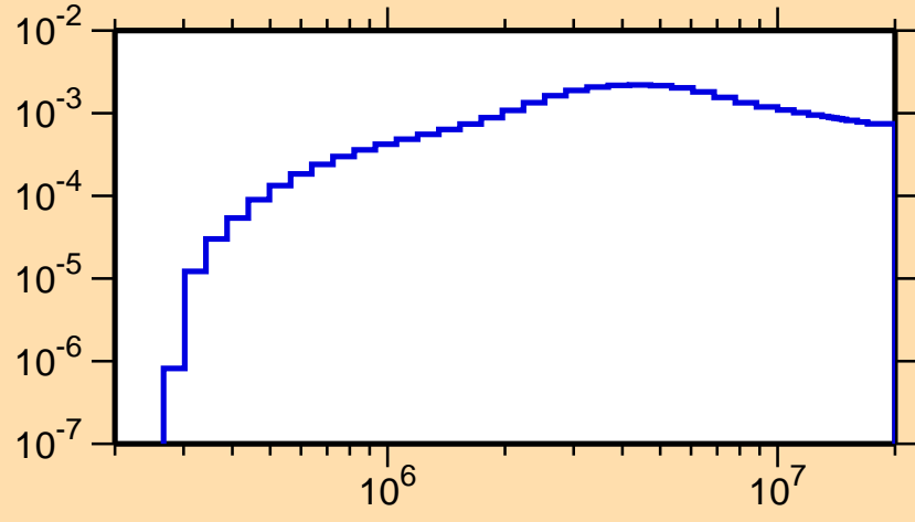
\sigma vs. E for ^{188}\text{Tl}(n,n_2)
