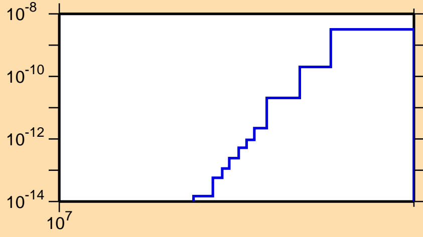
\sigma vs. E for ^{188}\text{Tl} (mt 34)
