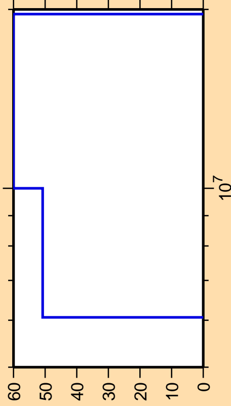
\Delta\sigma/\sigma vs. E for ^{188}\text{Tl} (mt 45)
