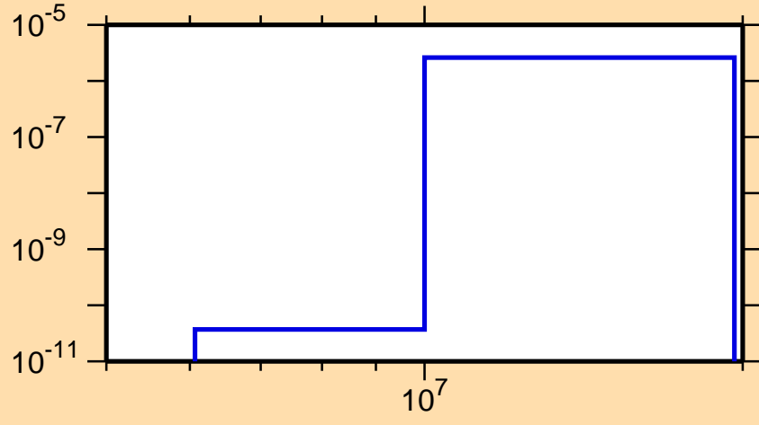
\sigma vs. E for ^{188}\text{Tl} (mt 45)
