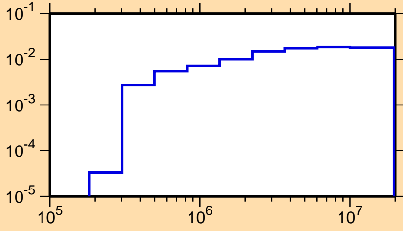
\sigma vs. E for ^{188}\text{Tl}(n,n_3)
