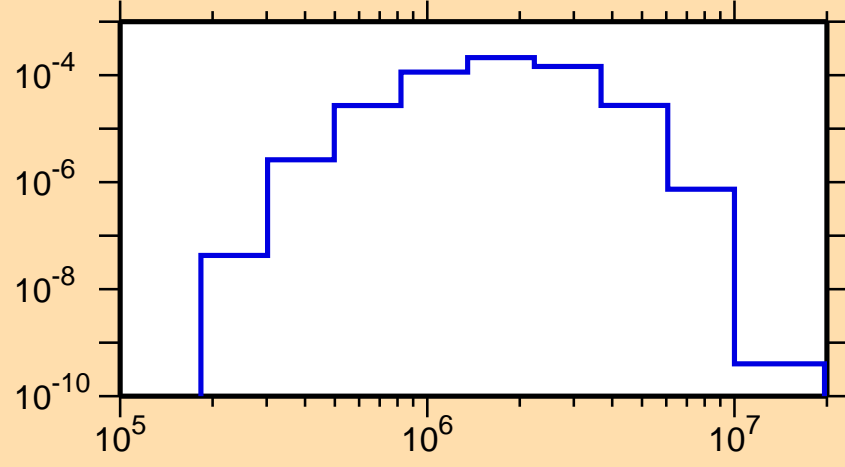
\sigma vs. E for ^{188}\text{Tl}(n,n_1)
