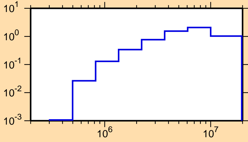
\sigma vs. E for ^{188}\text{Tl}(n,n\text{cont.})
