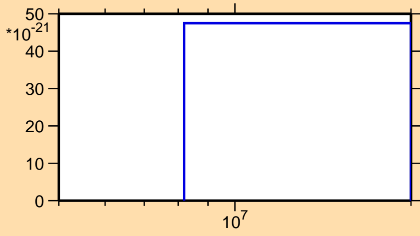
\sigma vs. E for ^{188}\text{Tl} (mt 42)
