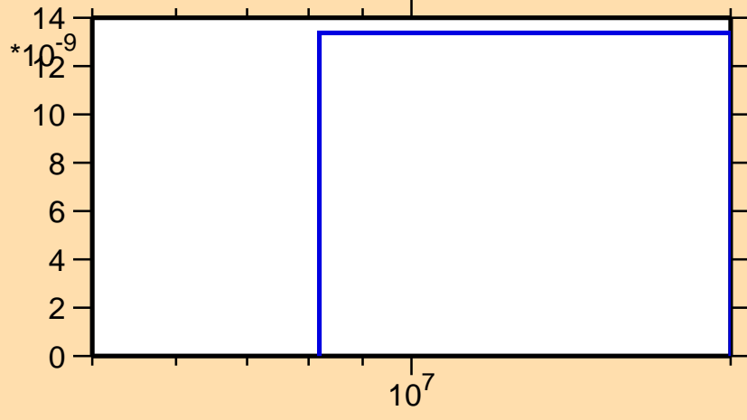
\sigma vs. E for ^{188}\text{Tl}(\text{mt117})
