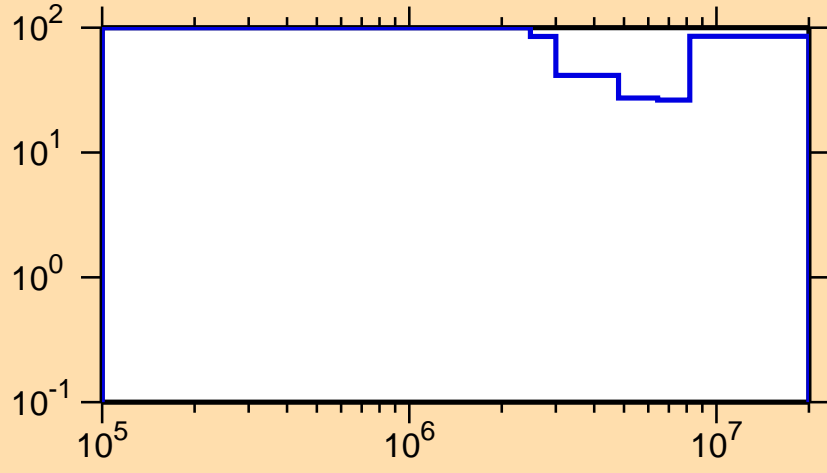
\Delta\sigma/\sigma vs. E for ^{188}\text{Tl}(n,ncont.)
