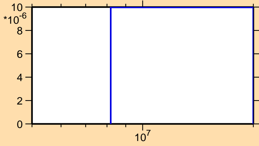
\sigma vs. E for ^{188}\text{Tl}(n,2n\alpha)
