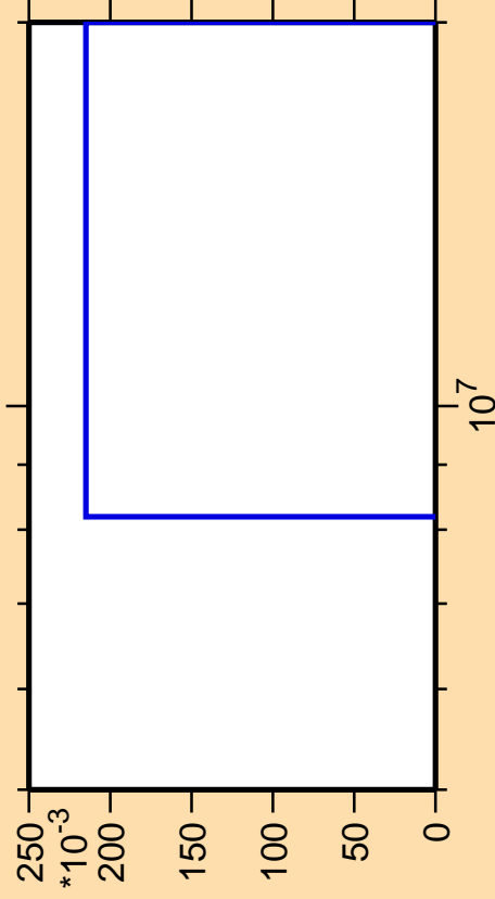
\Delta\sigma/\sigma vs. E for ^{189}\text{Tl}(\text{mt } 34)
