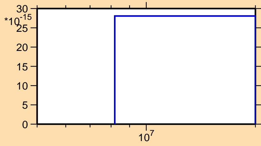
\sigma vs. E for ^{189}\text{Tl}(\text{mt } 34)
