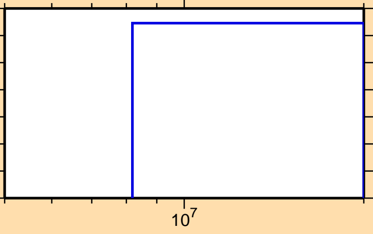
\sigma vs. E for ^{189}\text{Tl}(n,\text{nd})
