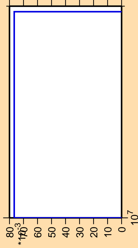
\Delta\sigma/\sigma vs. E for ^{189}\text{Tl}(n,\text{pt})
