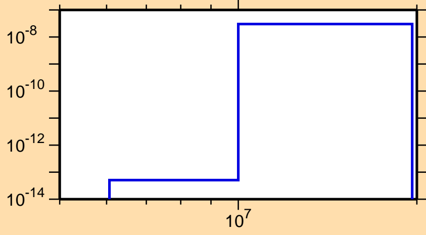
\sigma vs. E for ^{189}\text{Tl} (mt 45)
