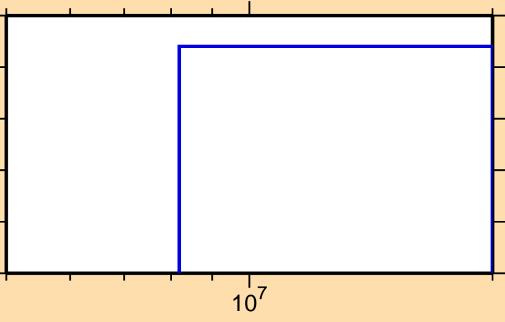
\sigma vs. E for ^{189}\text{Tl}(n,\text{nd})
