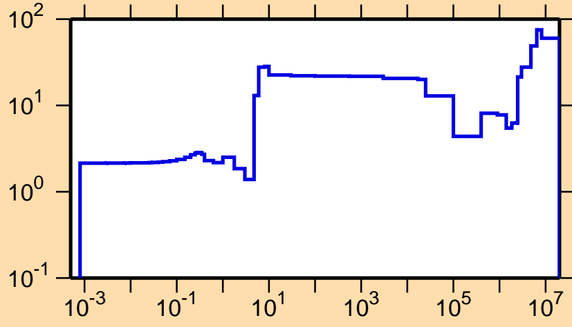
\Delta\sigma/\sigma vs. E for ^{189}\text{Tl}(n,el.)
