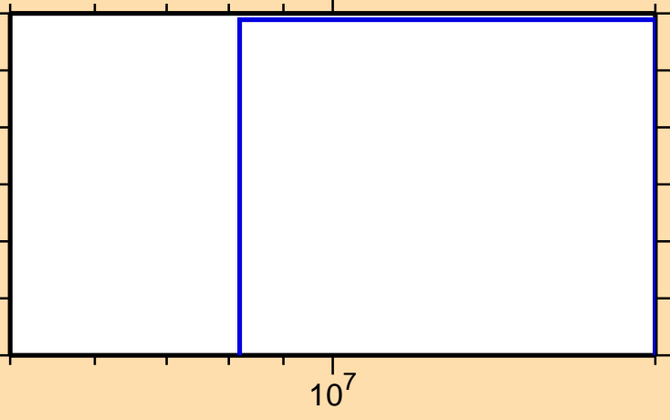
\sigma vs. E for ^{189}\text{Tl}(\text{mt117})
