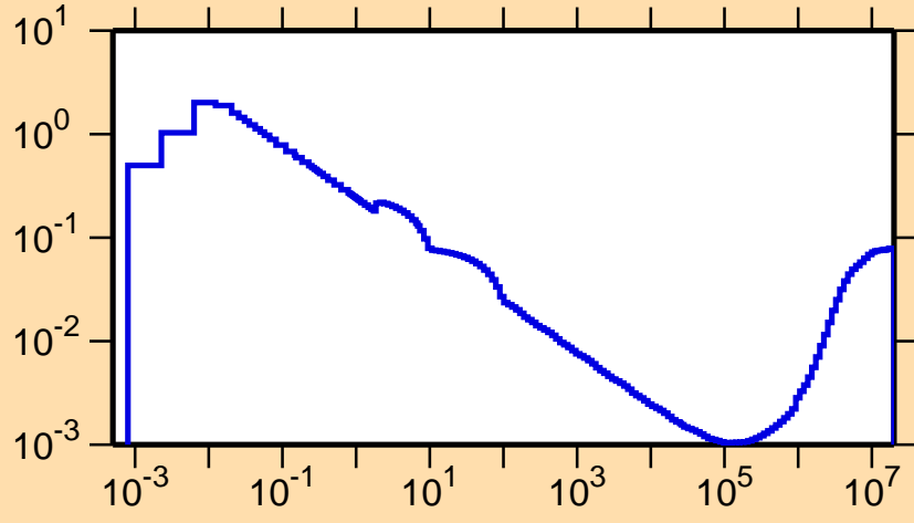
\sigma vs. E for ^{190}\text{Tl}(n,p)
