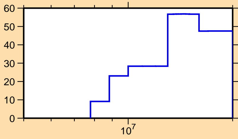
\Delta\sigma/\sigma vs. E for ^{190}\text{Tl}(n,\text{inel.})
