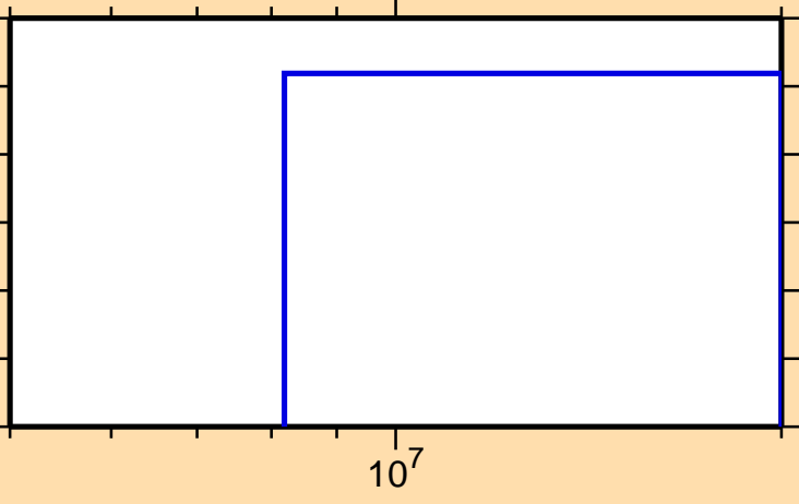
\sigma vs. E for ^{190}\text{Tl}(n,2np)
