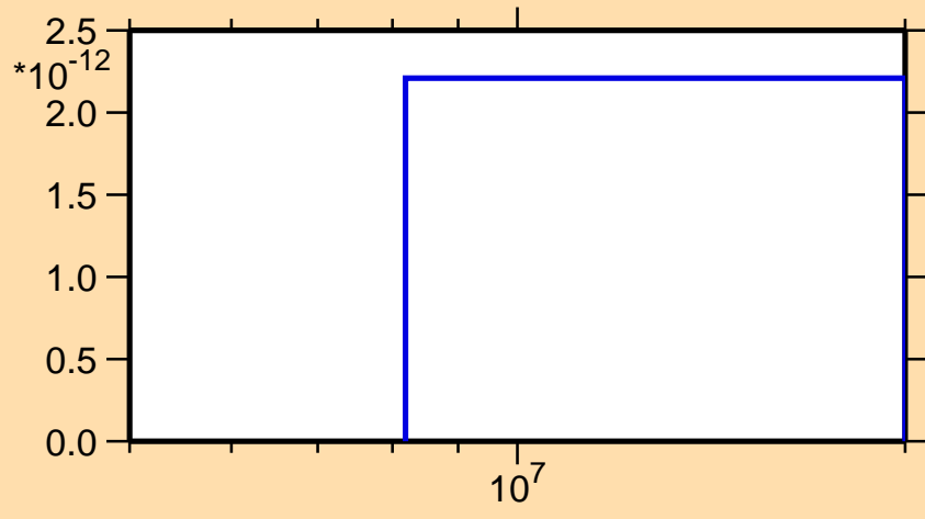
\sigma vs. E for ^{190}\text{Tl} (mt 34)
