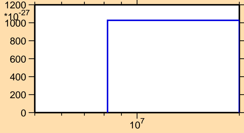
\sigma vs. E for ^{190}\text{Tl} (mt 42)
