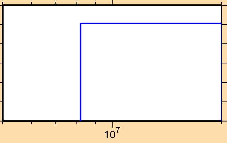
\sigma vs. E for ^{190}\text{Tl}(\text{mt117})
