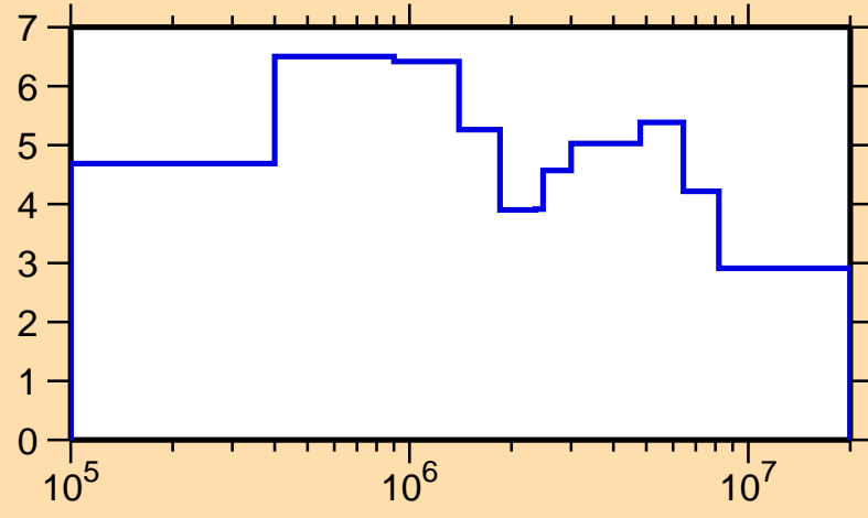
\Delta\sigma/\sigma vs. E for ^{190}\text{Tl}(n,\text{tot.})
