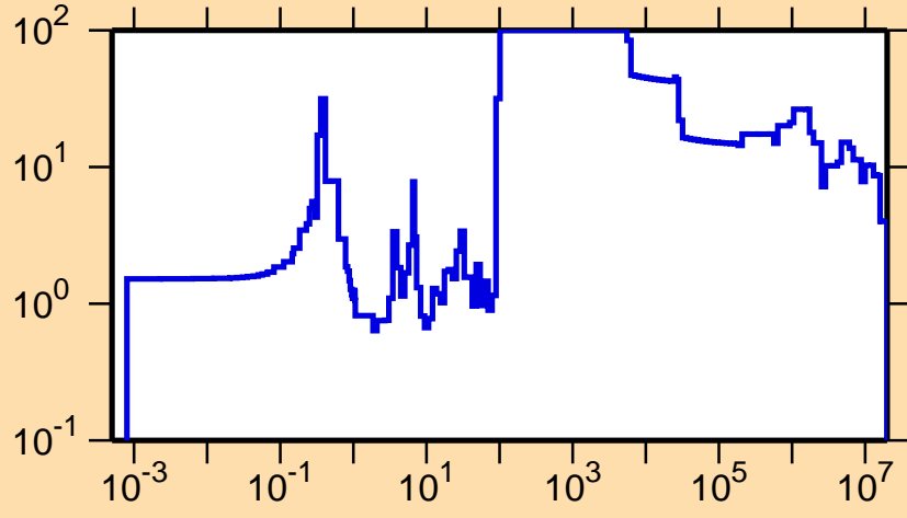
\Delta\sigma/\sigma vs. E for ^{191}\text{Tl}(n,el.)
