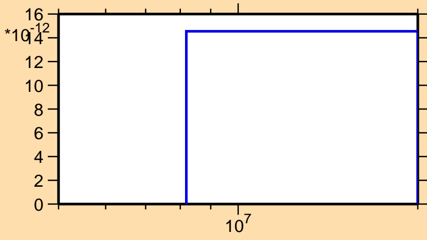
\sigma vs. E for ^{191}\text{Tl}(n,\text{pd})
