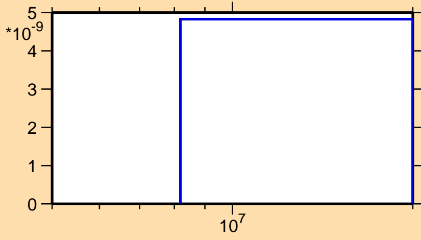
\sigma vs. E for ^{191}\text{Tl} (mt 45)
