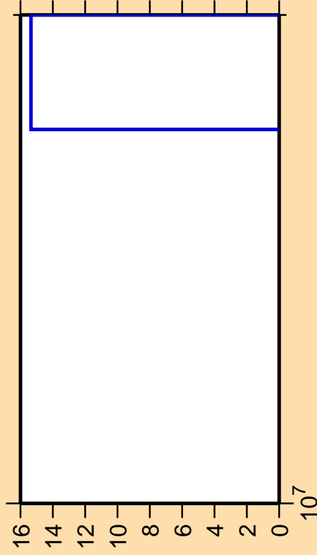
\Delta\sigma/\sigma vs. E for ^{192}\text{Tl} (mt 34)
