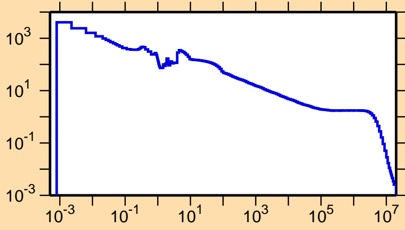
\sigma vs. E for ^{192}\text{Tl}(n,\gamma)
