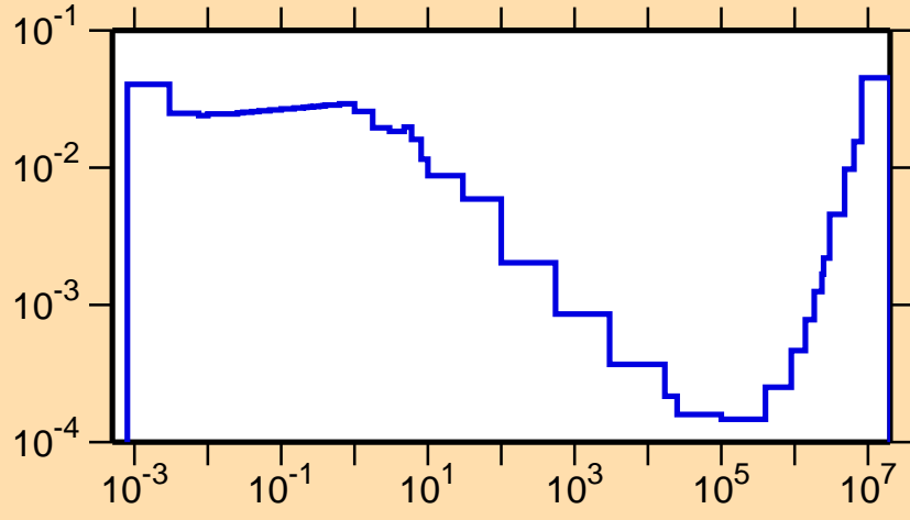
\sigma vs. E for ^{192}\text{Tl}(n,p)
