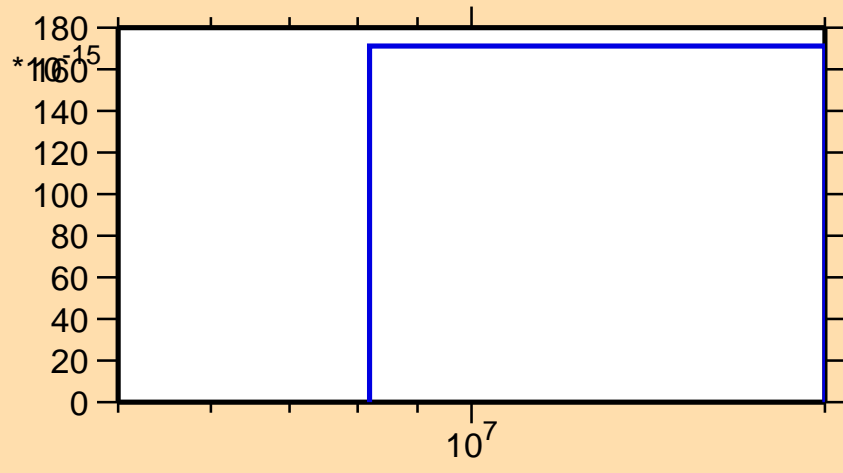
\sigma vs. E for ^{192}\text{Tl}(\text{mt } 34)
