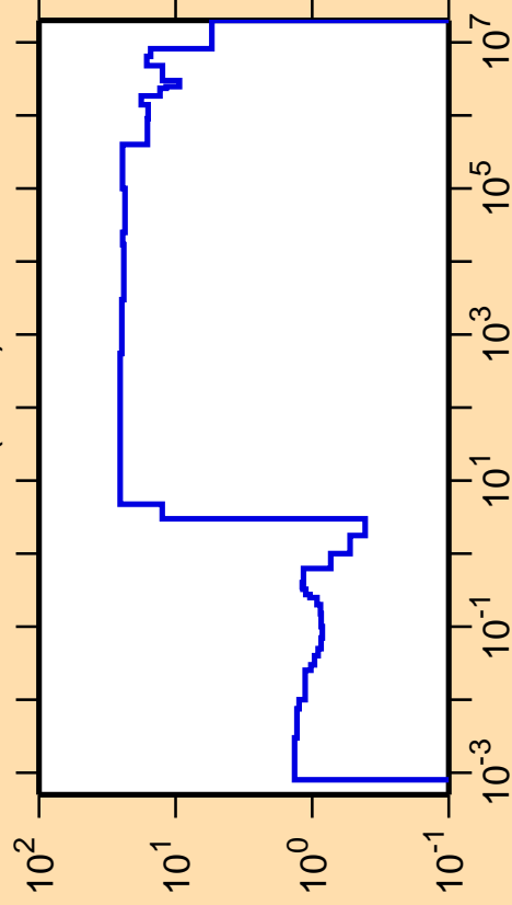
\Delta\sigma/\sigma vs. E for ^{192}\text{Tl}(n,\text{el.})
