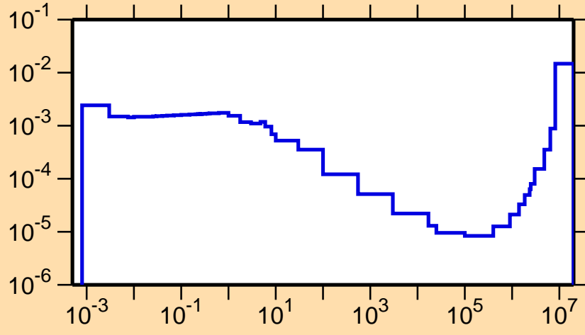
\sigma vs. E for ^{192}\text{Tl}(n,\alpha)
