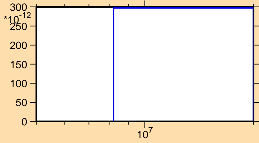
\sigma vs. E for ^{192}\text{Tl} (mt 45)
