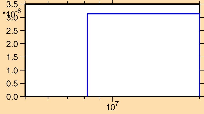
\sigma vs. E for ^{192}\text{Tl}(n,3n)
