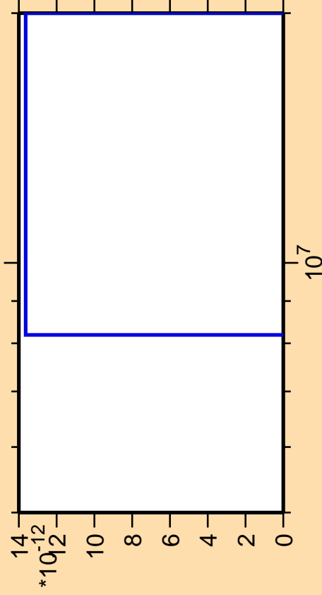
\Delta\sigma/\sigma vs. E for ^{192}\text{Tl} (mt 42)
