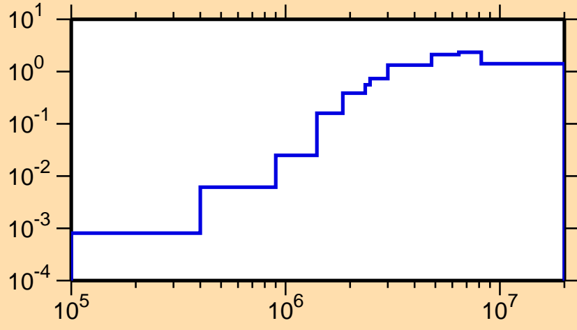
\sigma vs. E for ^{192}\text{Tl}(n,n\text{cont.})
