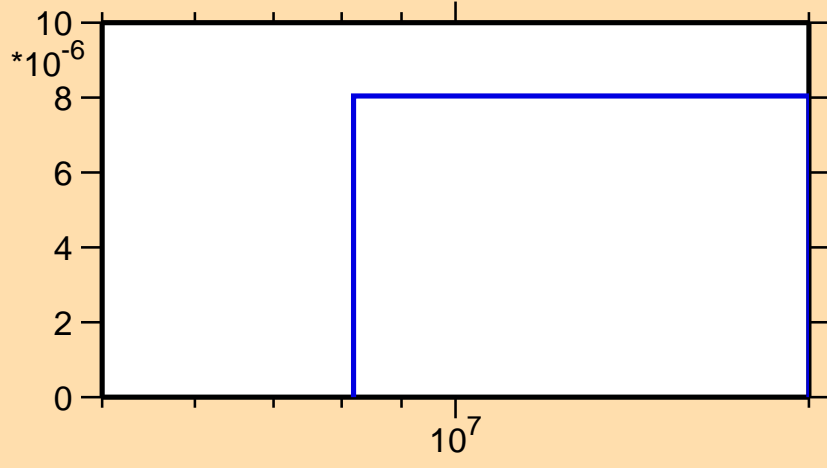
\sigma vs. E for ^{192}\text{Tl}(n,2np)
