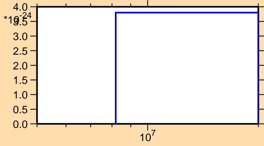
\sigma vs. E for ^{192}\text{Tl} (mt 42)
