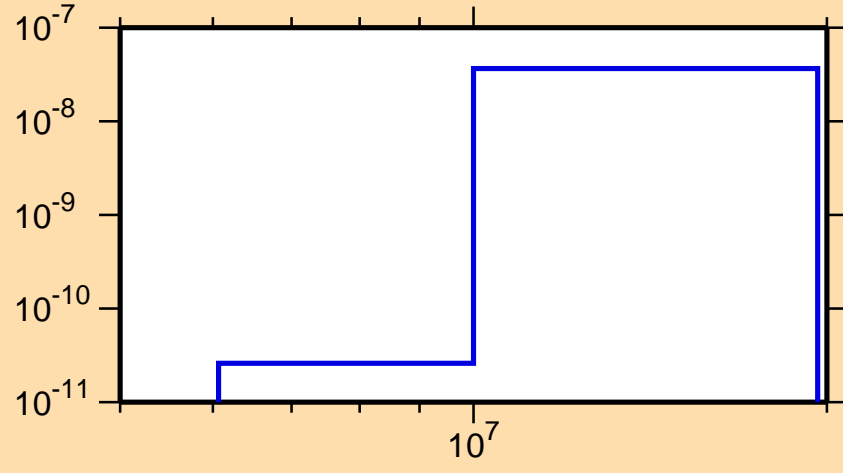
\sigma vs. E for ^{194}\text{Tl}(n,p\alpha)
