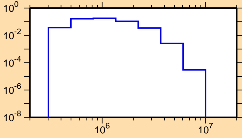
\sigma vs. E for ^{195}\text{Tl}(n,n_1)
