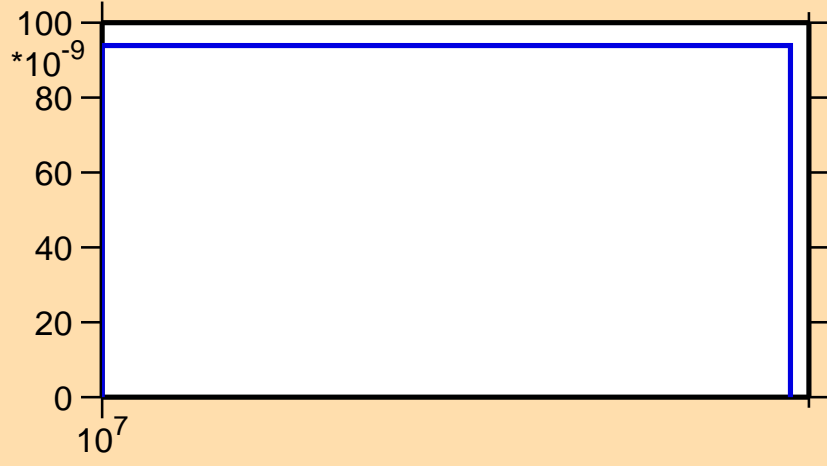
\sigma vs. E for ^{195}\text{Tl}(n,2np)
