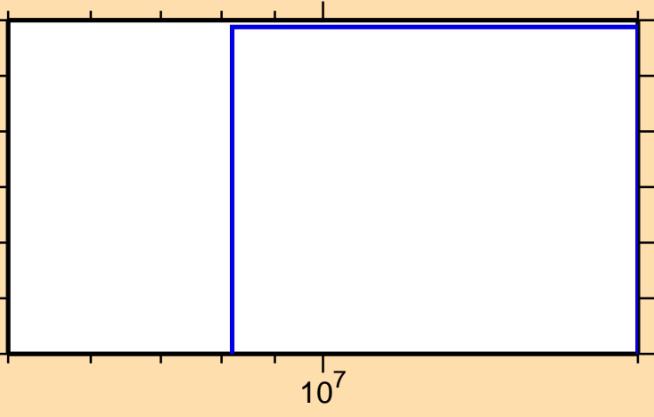
\sigma vs. E for ^{195}\text{Tl}(n,\text{nd})
