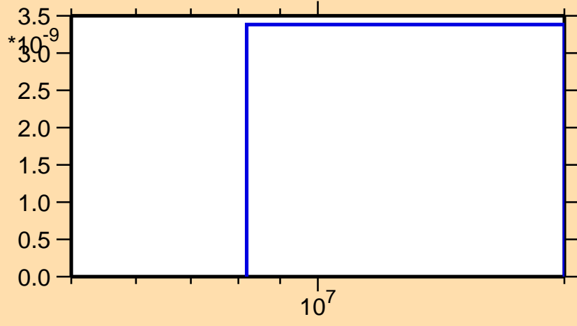
\sigma vs. E for ^{195}\text{Tl}(n,\text{He3})
