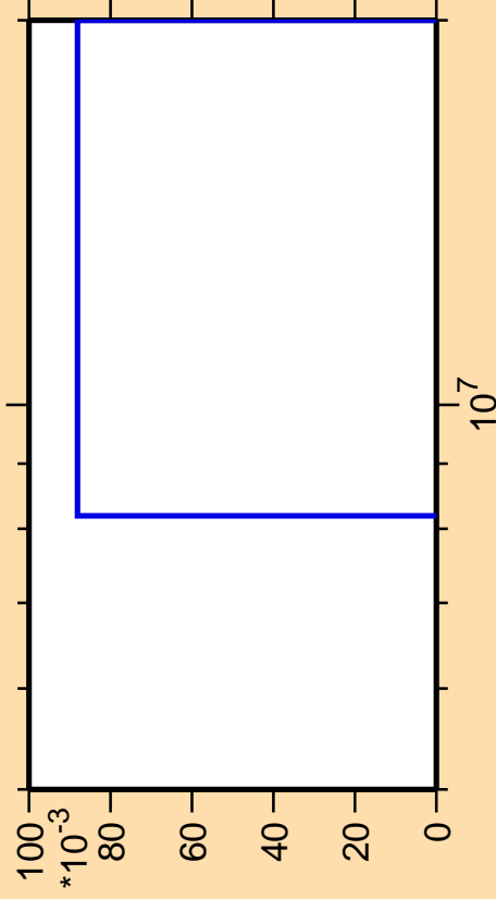
\Delta\sigma/\sigma vs. E for ^{195}\text{Tl} (mt 45)
