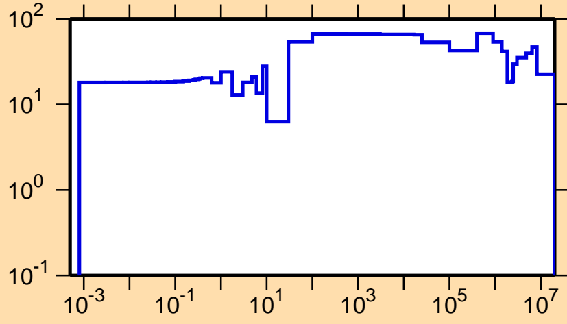
\Delta\sigma/\sigma vs. E for ^{195}\text{Tl}(n,el.)
