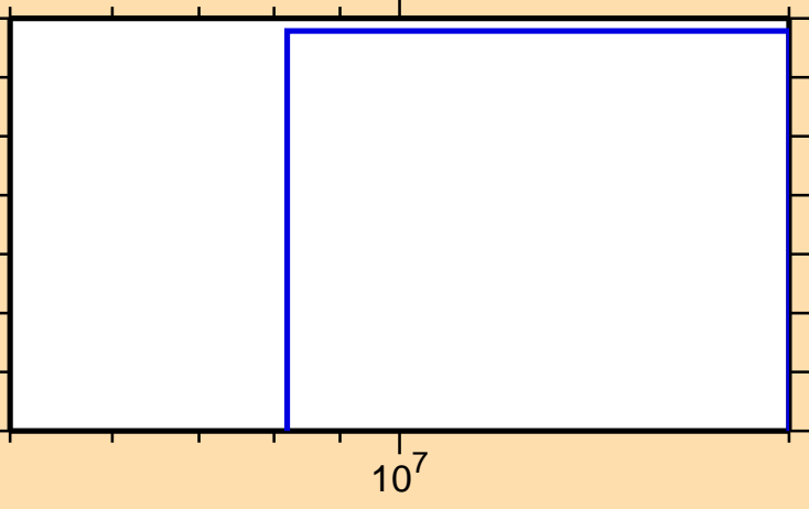
\sigma vs. E for ^{195}\text{Tl} (mt 45)
