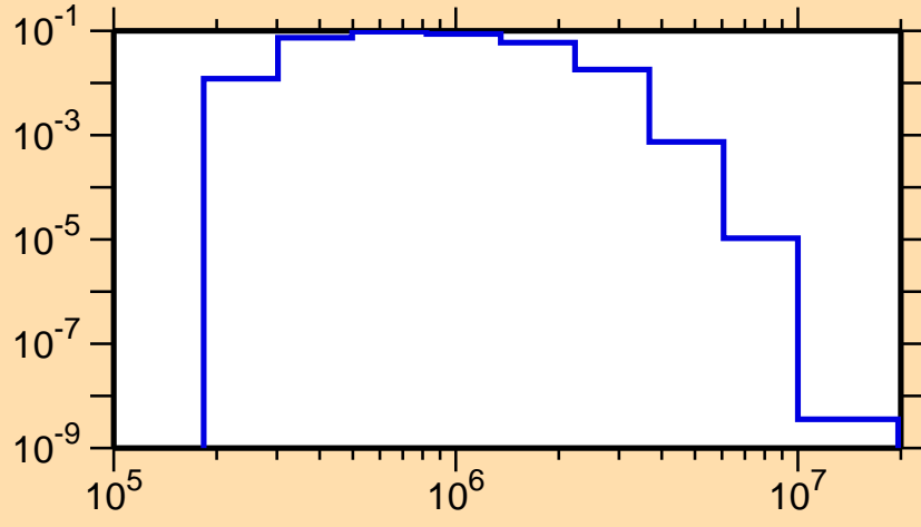
\sigma vs. E for ^{196}\text{Tl}(n,n_2)
