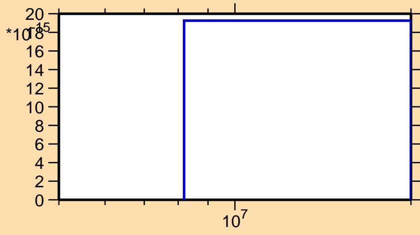
\sigma vs. E for ^{196}\text{Tl}(\text{mt } 45)
