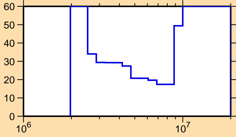
\Delta\sigma/\sigma vs. E for ^{197}\text{Tl}(n,n\text{cont.})
