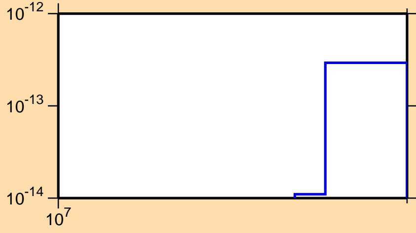
\sigma vs. E for ^{197}\text{Tl} (mt 45)
