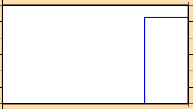
\sigma vs. E for ^{197}\text{Tl} (mt 42)
