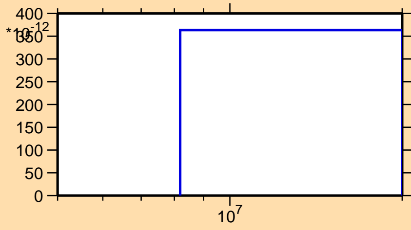
\sigma vs. E for ^{198}\text{Tl}(n,nt)
