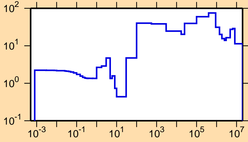
\Delta\sigma/\sigma vs. E for ^{198}\text{Tl}(n,el.)
