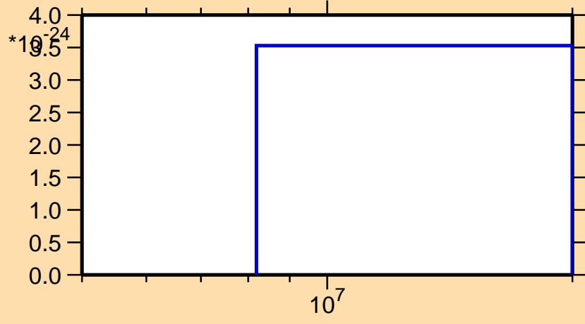
\sigma vs. E for ^{198}\text{Tl} (mt 42)
