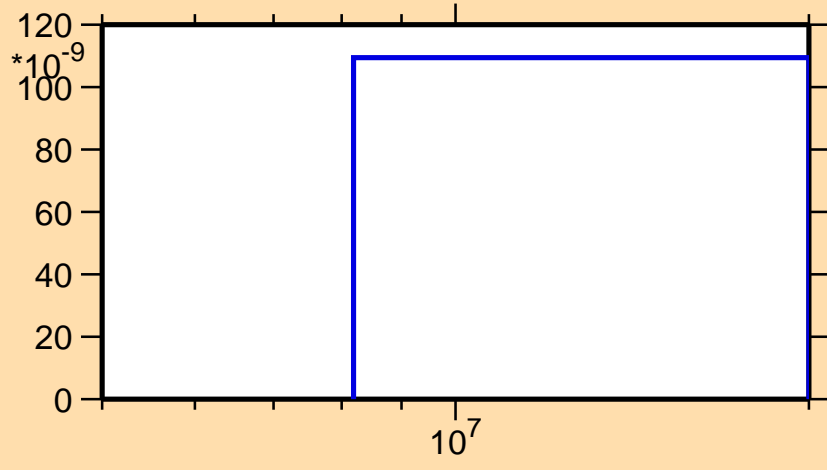
\sigma vs. E for ^{198}\text{Tl}(n,nd)
