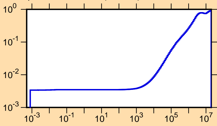
\mu vs. E for ^{199}\text{Tl}(\text{mt251})
