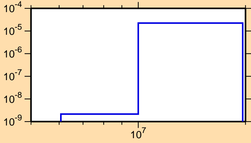
\sigma vs. E for ^{199}\text{Tl}(n,n\alpha)
