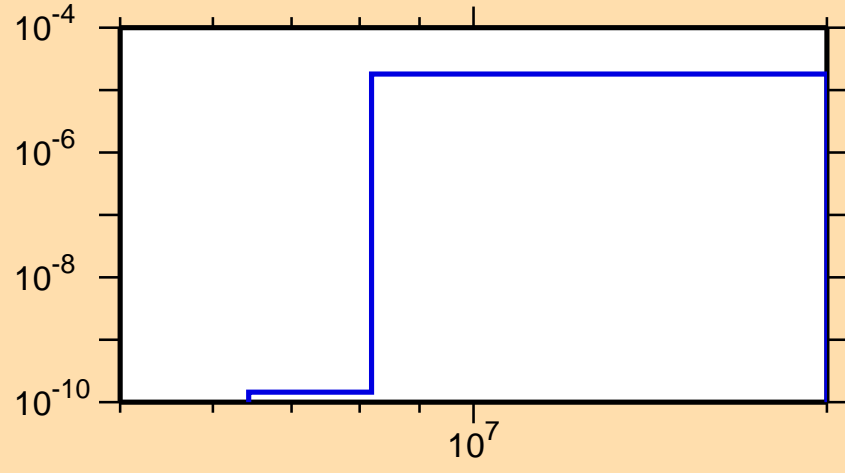
\sigma vs. E for ^{199}\text{Tl}(n,n\alpha)
