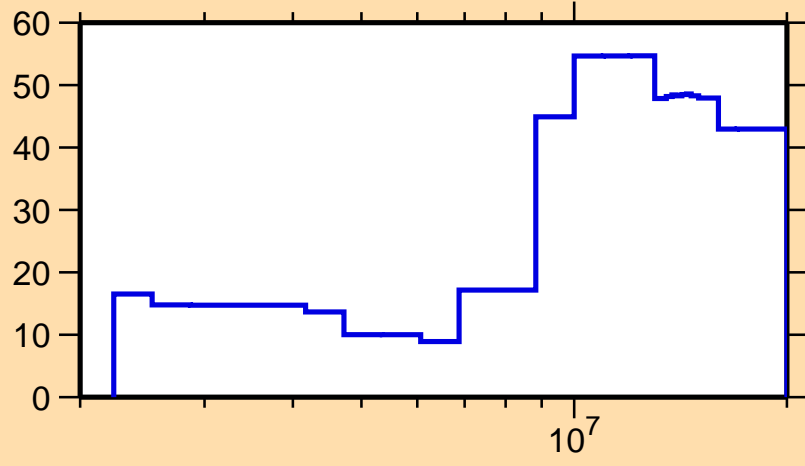
\Delta\sigma/\sigma vs. E for ^{200}\text{Tl}(n,n\text{cont.})
