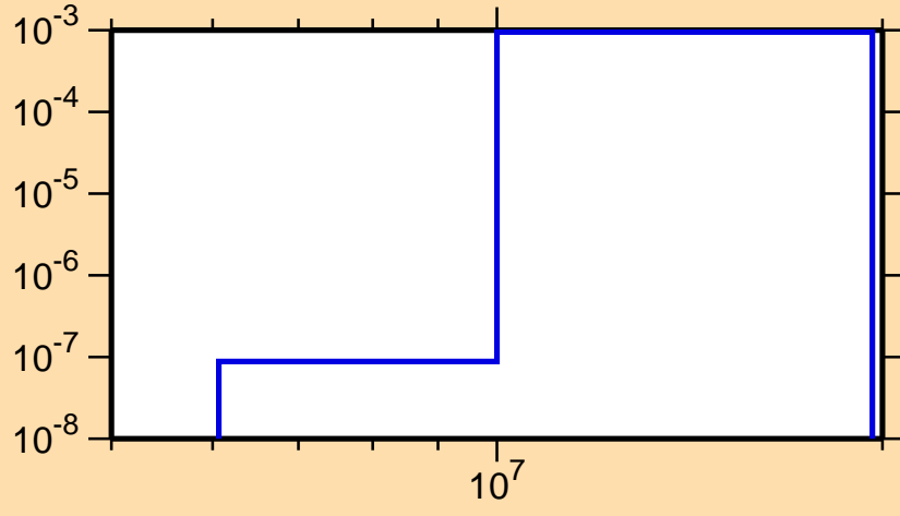
\sigma vs. E for ^{200}\text{Tl}(n,np)
