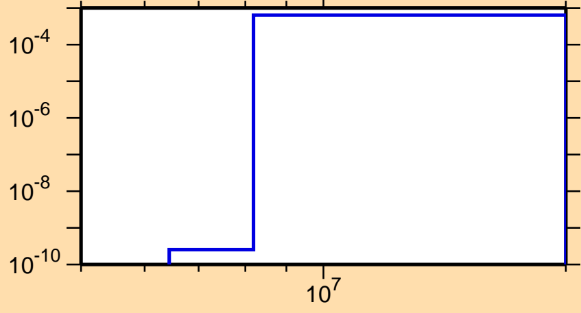
\sigma vs. E for ^{200}\text{Tl}(n,d)
