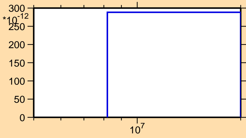
\sigma vs. E for ^{200}\text{Tl}(n,2n\alpha)
