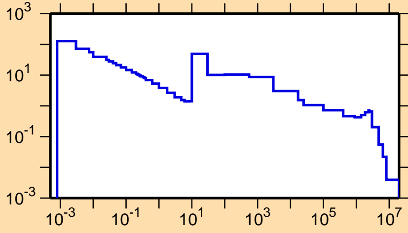
\sigma vs. E for ^{200}\text{Tl}(n,\gamma)
