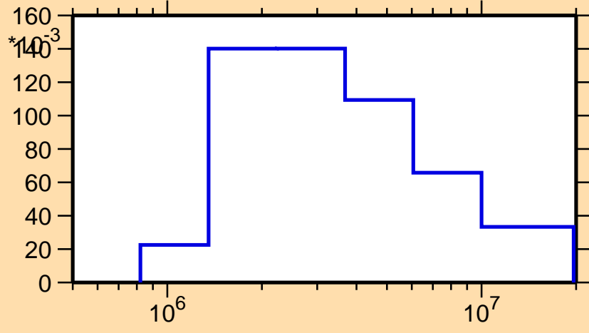
\sigma vs. E for ^{201}\text{Tl}(n,n_4)
