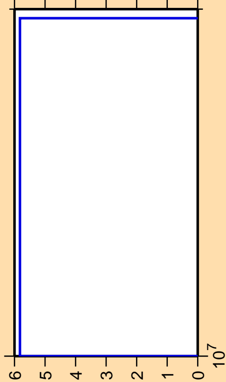
\Delta\sigma/\sigma vs. E for ^{201}\text{Tl}(n,\text{He}3)
