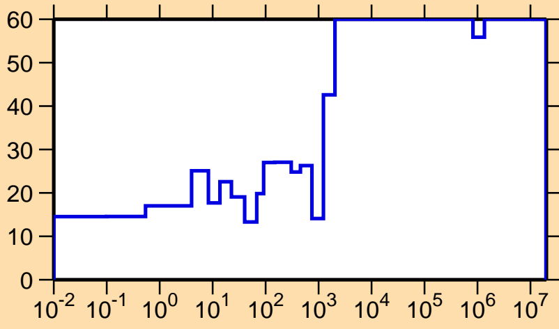
\Delta\sigma/\sigma vs. E for ^{201}\text{Tl}(n,\gamma)
