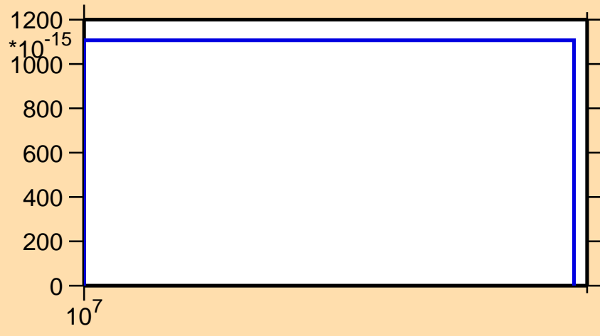
\sigma vs. E for ^{201}\text{Tl}(n,\text{He}3)
