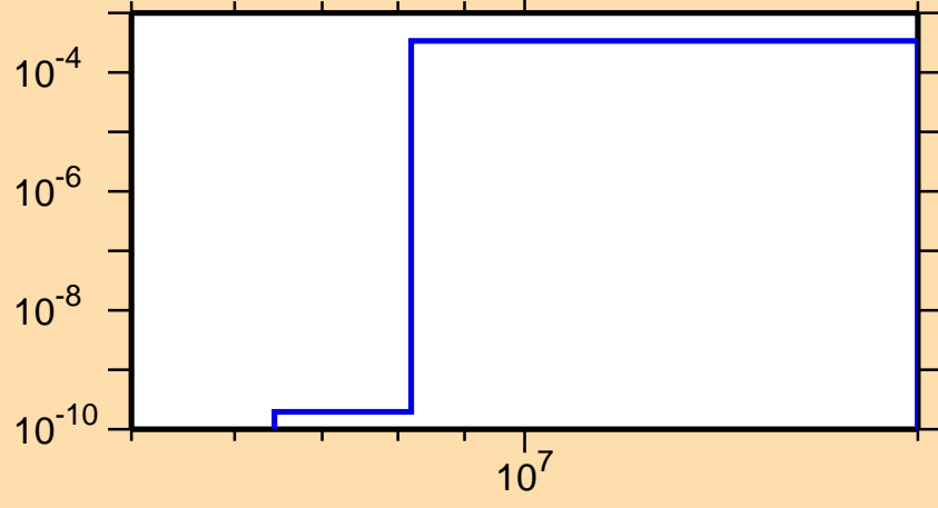
\sigma vs. E for ^{201}\text{Tl}(n,d)
