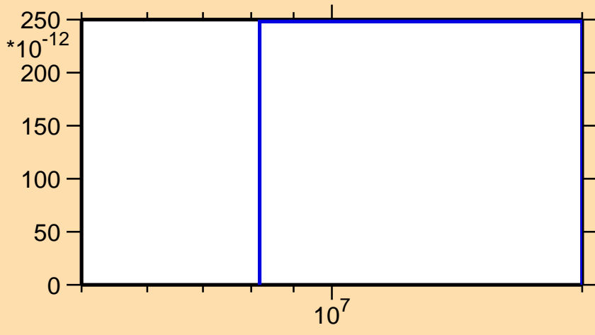
\sigma vs. E for ^{201}\text{Tl}(n,nt)
