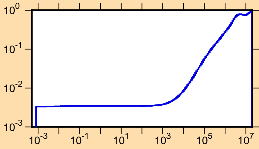
\mu vs. E for ^{202}\text{Tl}(\text{mt251})
