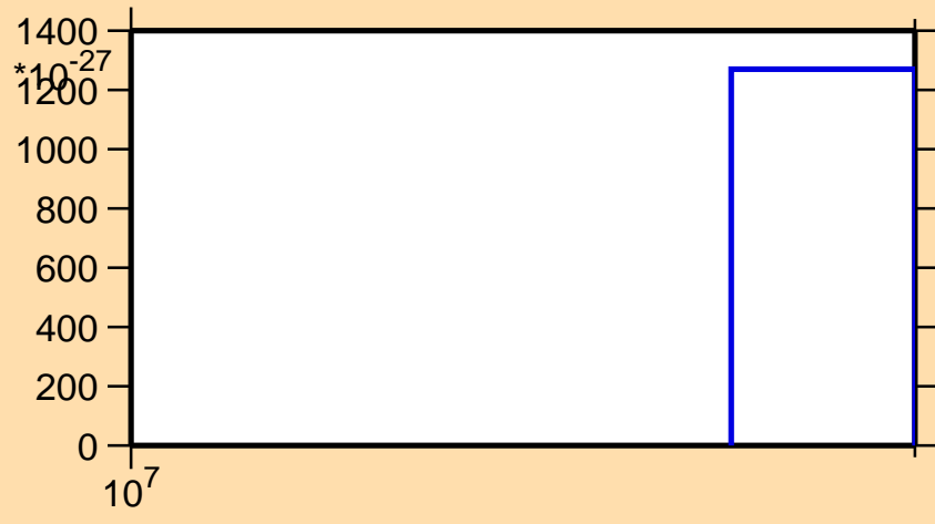
\sigma vs. E for ^{202}\text{Tl} (mt 42)
