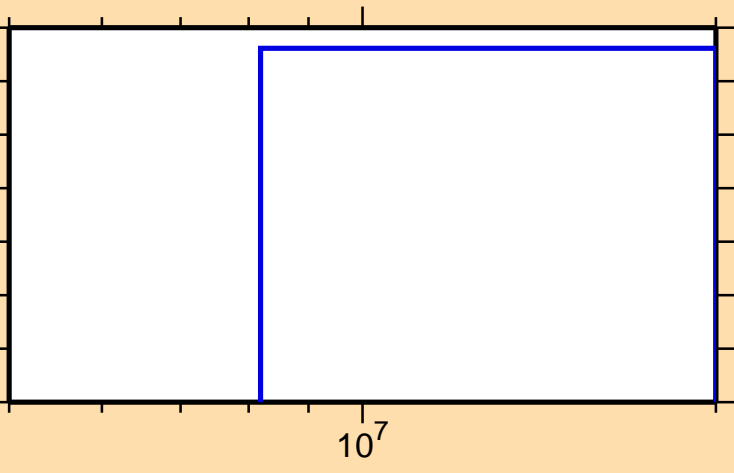
\sigma vs. E for ^{202}\text{Tl}(n,2np)
