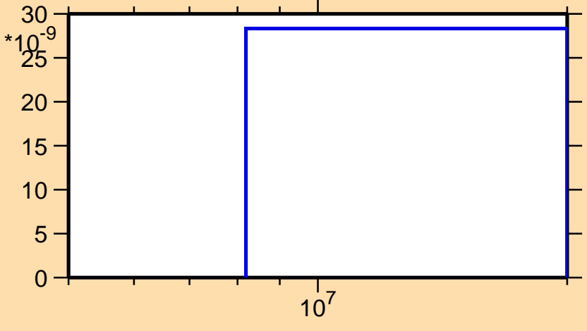
\sigma vs. E for ^{202}\text{Tl}(n,nd)
