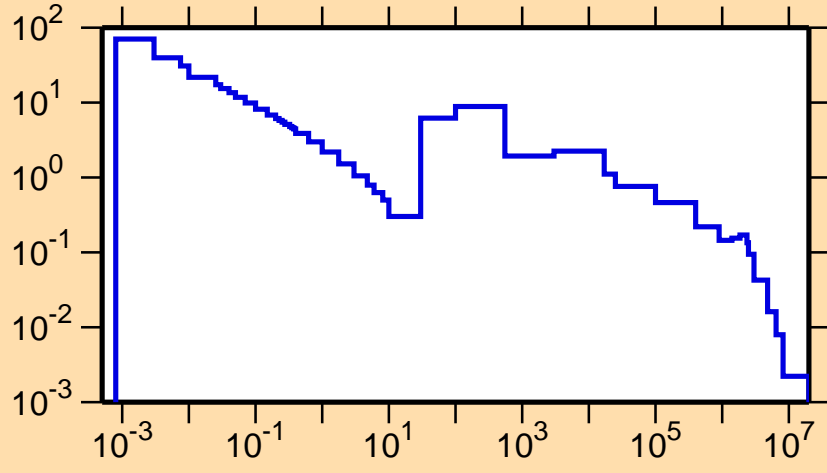
\sigma vs. E for ^{202}\text{Tl}(n,\gamma)
