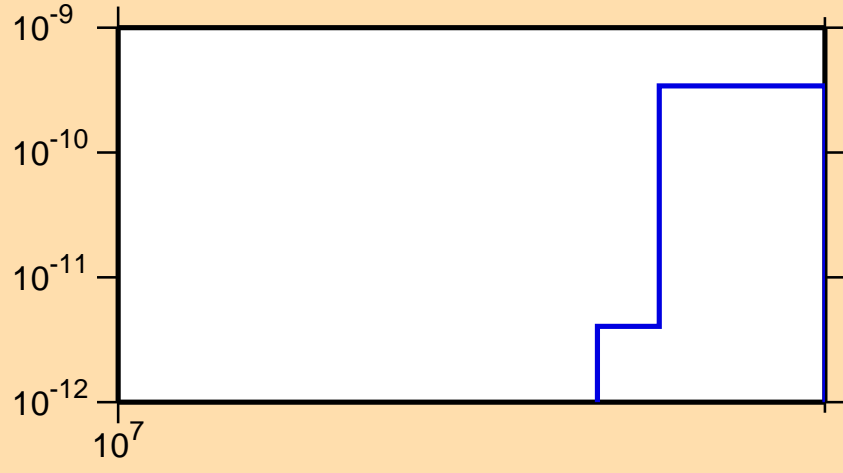
\sigma vs. E for ^{203}\text{Tl}(n,2n\alpha)
