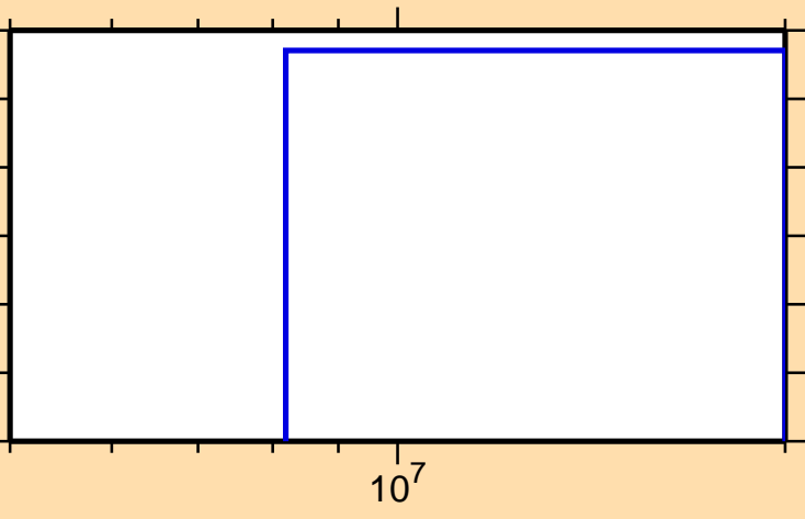
\sigma vs. E for ^{203}\text{Tl}(n,nt)
