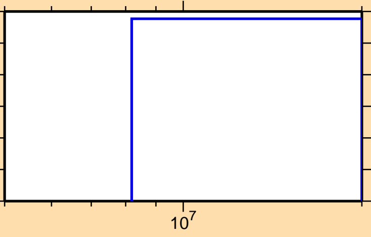
\sigma vs. E for ^{203}\text{Tl}(n,t)
