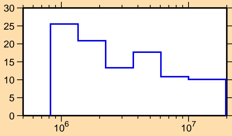
\Delta\sigma/\sigma vs. E for ^{204}\text{Tl}(n,\text{el.})
