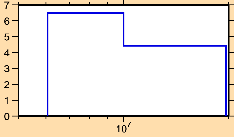
\Delta\sigma/\sigma vs. E for ^{204}\text{Tl}(n,\text{tot.})
