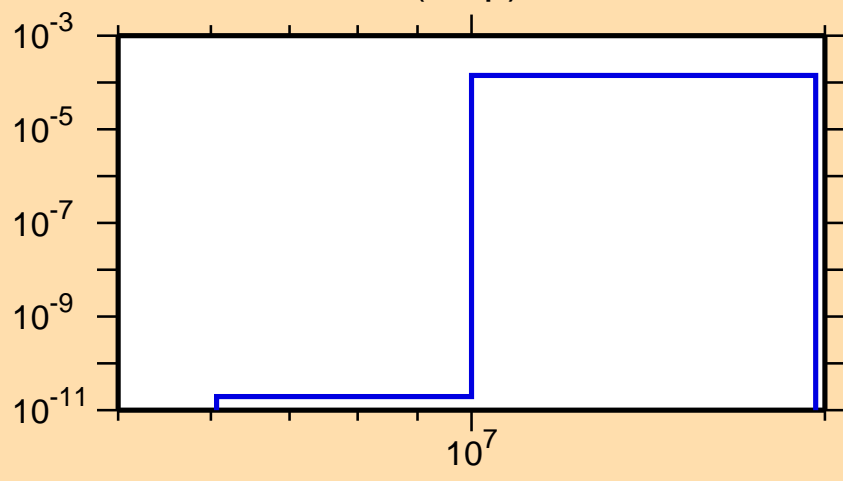
\sigma vs. E for ^{204}\text{Tl}(n,np)
