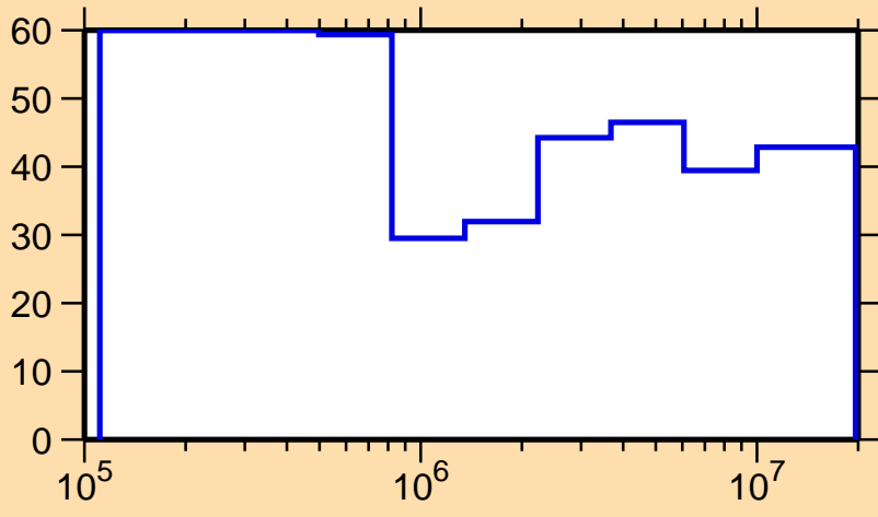
\Delta\sigma/\sigma vs. E for ^{204}\text{Tl}(n,n_1)
