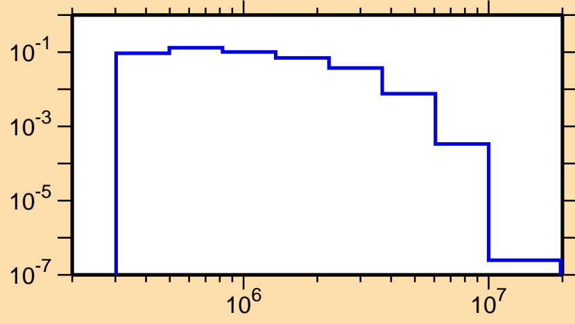
\sigma vs. E for ^{204}\text{Tl}(n,n_3)
