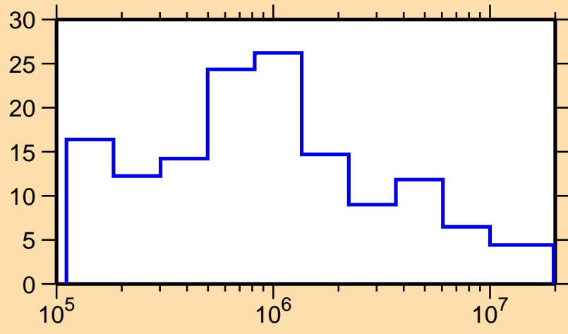
\Delta\sigma/\sigma vs. E for ^{204}\text{Tl}(n,\text{tot.})
