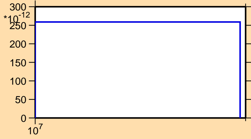
\sigma vs. E for ^{204}\text{Tl}(n,nt)
