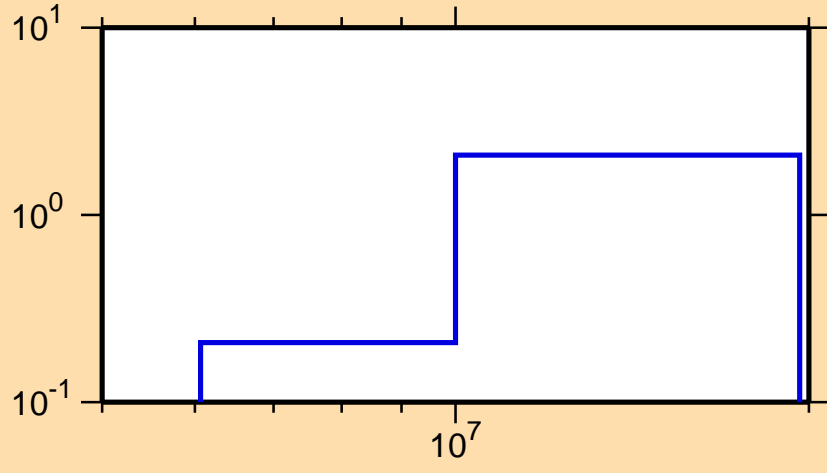
\sigma vs. E for ^{204}\text{Tl}(n,2n)
