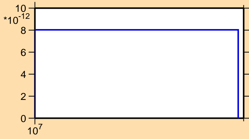
\sigma vs. E for ^{204}\text{Tl}(n,2n\alpha)
