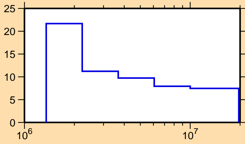
\Delta\sigma/\sigma vs. E for ^{204}\text{Tl}(n,\text{nonel.})
