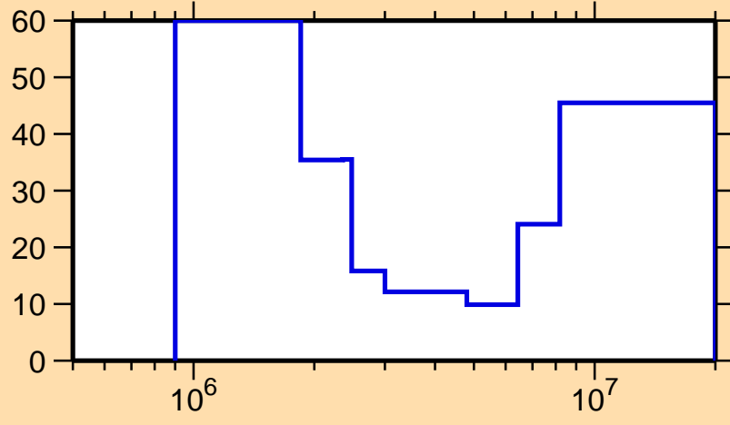
\Delta\sigma/\sigma vs. E for ^{204}\text{Tl}(n,ncont.)
