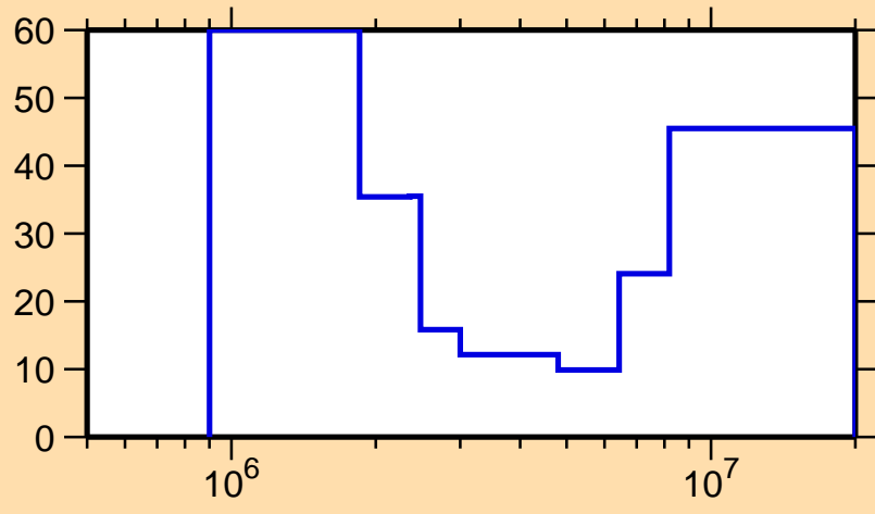
\Delta\sigma/\sigma vs. E for ^{204}\text{Tl}(n,n\text{cont.})
