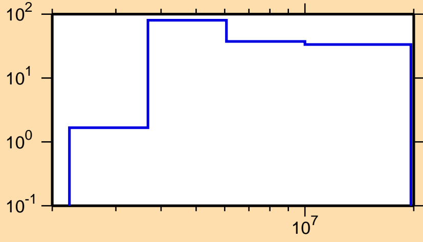
\Delta\sigma/\sigma vs. E for ^{205}\text{Tl}(n,p)
