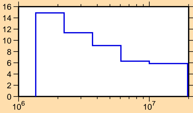
\Delta\sigma/\sigma vs. E for ^{205}\text{Tl}(n,n\text{nonel.})
