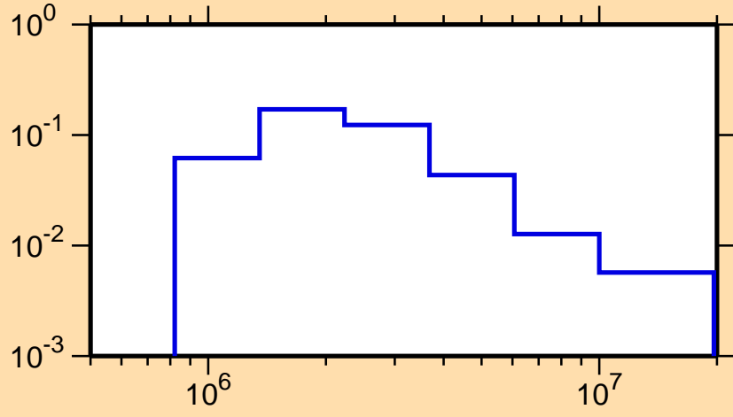
\sigma vs. E for ^{205}\text{Tl}(n,n_3)
